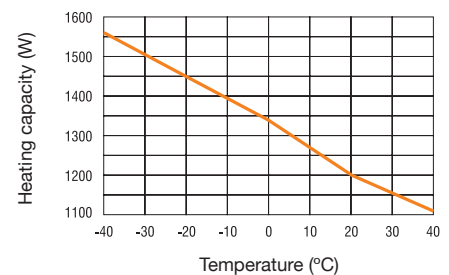
Heating capacity / Ambient temperature diagram CS 030
