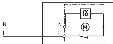
Connection diagram
