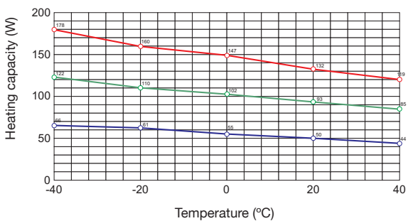
Heating capacity / Ambient temperature diagram CS 060
