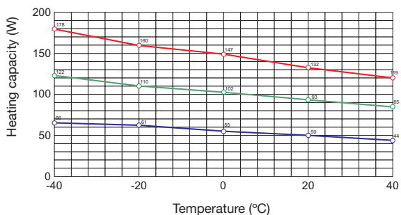
Heating capacity / Ambient temperature diagram CS 060
